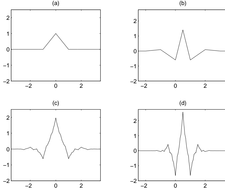
Figure 3: The piece-wise linear spline biorthogonal system. (a): The scaling function, \varphi . (b): The wavelet, \psi . (c): The dual scaling function, \tilde{\varphi} . (d): The dual wavelet, \tilde{\psi} .
