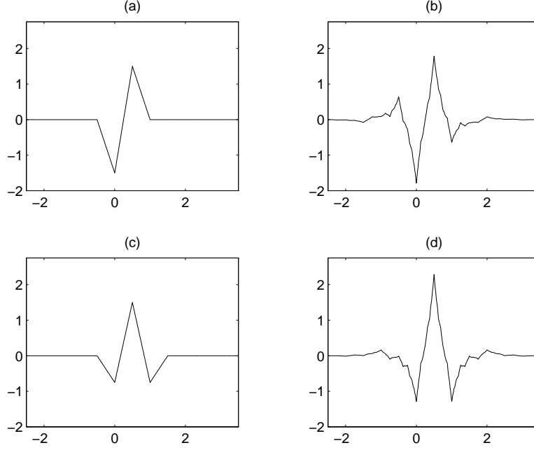
Figure 4: Examples of spline à trous wavelets. (a): The wavelet, \phi^C . (b): The dual wavelet, \tilde{\phi}^C . (c): The wavelet, \phi^D . (d): The dual wavelet, \tilde{\phi}^D .
