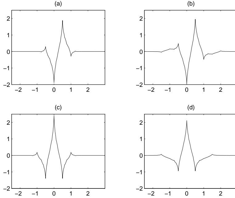
Figure 2: Examples of Burt-Adelson à trous wavelets. (a): The wavelet, \phi^A . (b): The dual wavelet, \tilde{\phi}^A . (c): The wavelet, \phi^B . (d): The dual wavelet, \tilde{\phi}^B .
