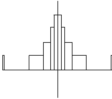
Diagram 2. The function D_4 .
