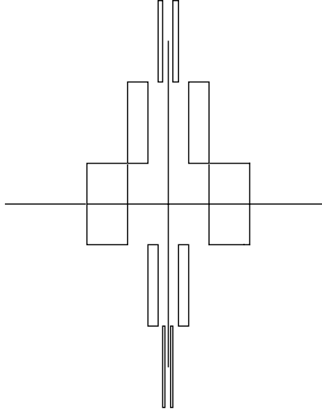
Fig. 1. Support of MSF wavelet for non-expansive dilation.
